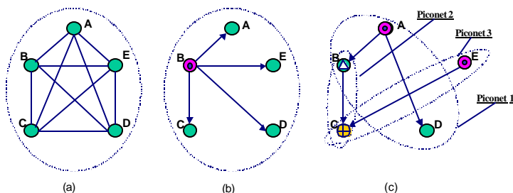
Figure 1: (a) Single channel model. (b),(c) Different configurations according to the Bluetooth multiple channel model.
