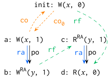
Fig. 11. Release-Acquire Visibility
