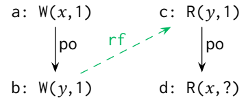
Fig. 1. Event Graph
