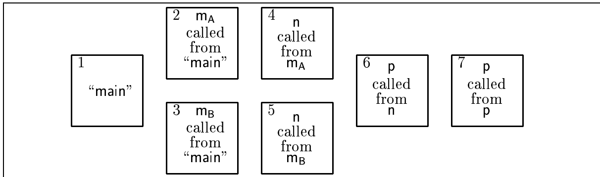
Figure 5: Trace graph nodes for the example program.
