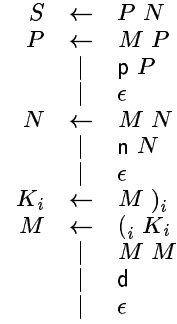
Figure 10: Grammar for CFL queries.
