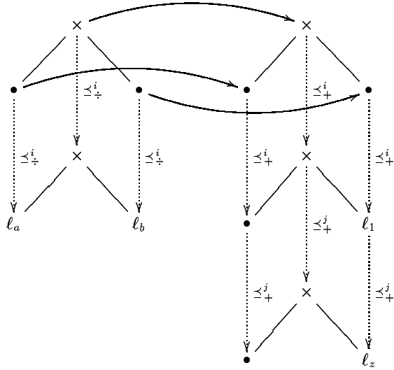
Flow graph G
