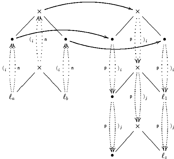
CFL Graph G_{CFL}
