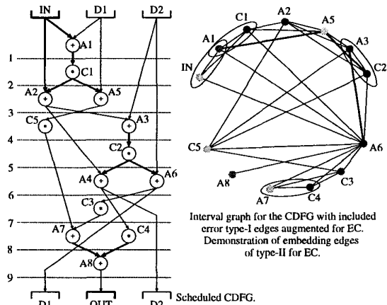
Figure 3: An example of addition of type-II constraints to the graph coloring problem for EC.
