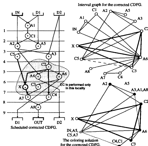
Figure 5: Individual steps in the post-processing for EC: graph bipartitioning, subgraph compression, and graph coloring on the compressed and updated interval graph.
