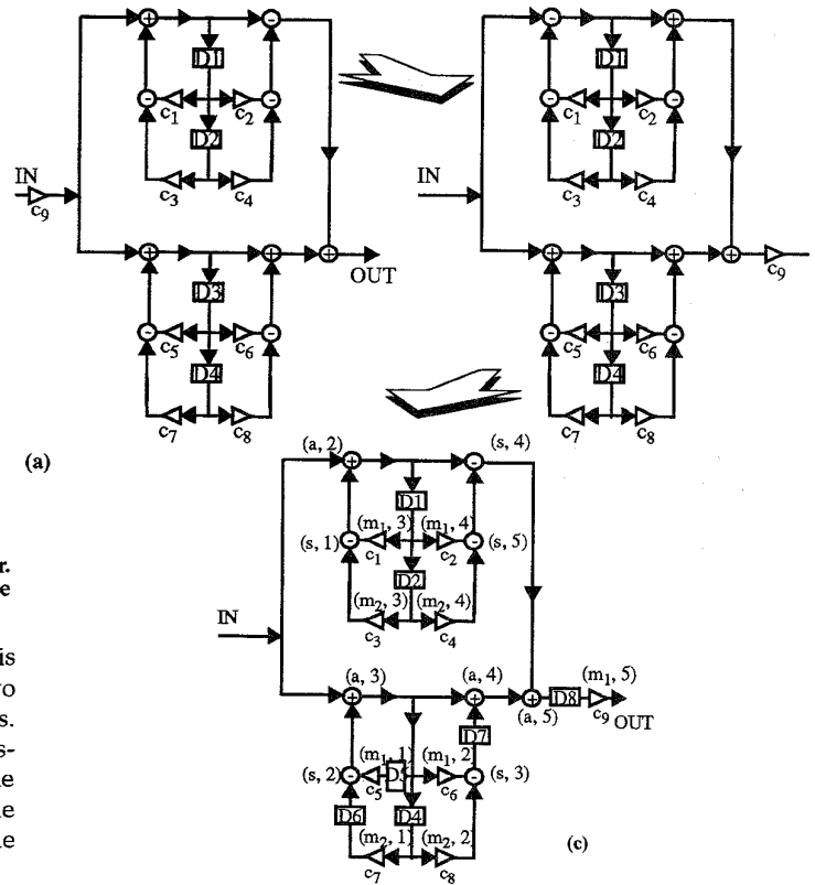
Fig. 3: The sequence of transformations for the simultaneous optimization of testability and area. First (a) associativity and the inverse element law are applied; next (b) scaling transformation; and (c) retiming. The corresponding datapath is shown in Fig. 4.
