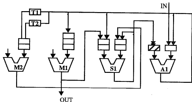
Fig. 4: The datapath of the transformed 4th order parallel IIR. Only one scan register (shaded) is required to break all loops in the datapath, compared with 4 scan register in the initial design.
