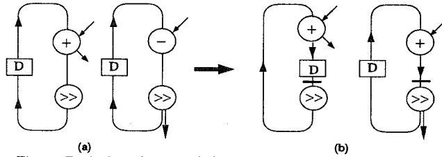
Fig. 6: Retiming for testability optimization. The crossed edges in the transformed CDFG are variables stored in the same scan register.
