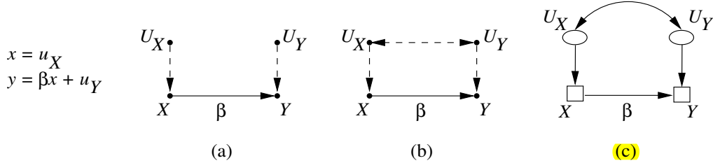
Figure 1: A simple structural equation model, and its associated diagrams, showing: (a) Independent unobserved exogenous variables (connected by dashed arrows) (b) Dependent exogenous variables and (c) an equivalent, more traditional notation, in which latent variables are enclosed in ovals.
