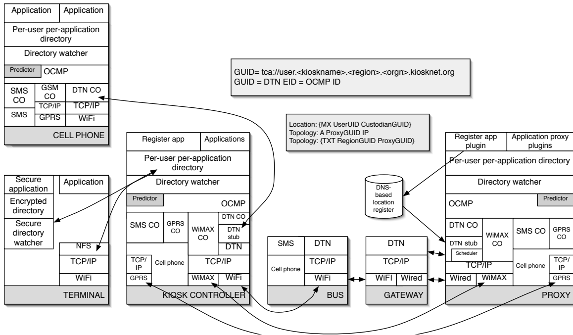
Figure 2: Software architecture.
