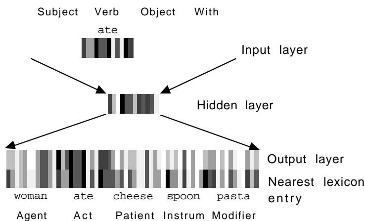
Figure 8: Expectations embedded in the word ate. The bottom layer shows the lexicon entries that are closest to the output generated by the network (Euclidian distance of normalized vectors). The effect is more pronounced when a small hidden layer is used. In this example, a network with 12 hidden units was trained for 50 epochs with a learning rate 0.1.
