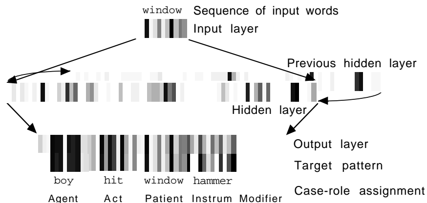
Figure 11: Snapshot of recurrent FGREP simulation. The network is in the middle of reading The boy hit the window with the hammer . The hidden layer pattern is saved after each step in the sequence, and used as input to the hidden layer during the next step, together with the actual input.
