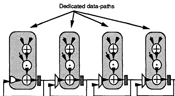
Figure 2: Cathedral-III architecture for the 16 tap symmetrical filter.
