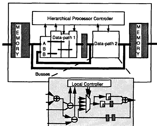
Figure 1: Processor architecture and a dedicated data-path.
