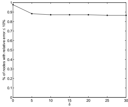
8.1: Temperature diffusion
