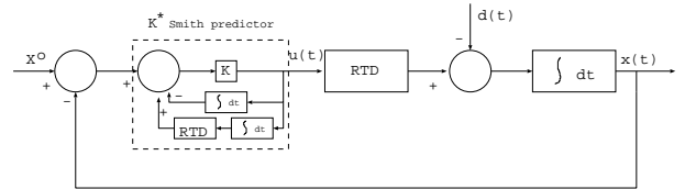
Figure 3: Queue dynamic model using a proportional controller plus a Smith Predictor
