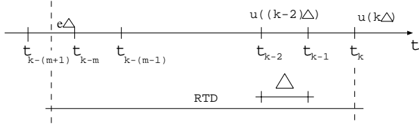
Figure 7: Discrete Time Notation
