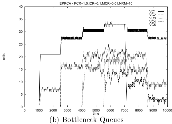
Figure 11: Aperiodic + Virtual Feedback
