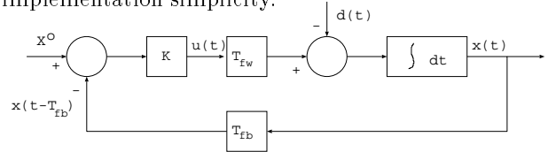
Figure 5: Queue dynamic model from the source point of view
