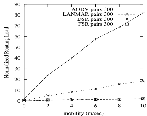
Fig. 3. Normalized routing load
