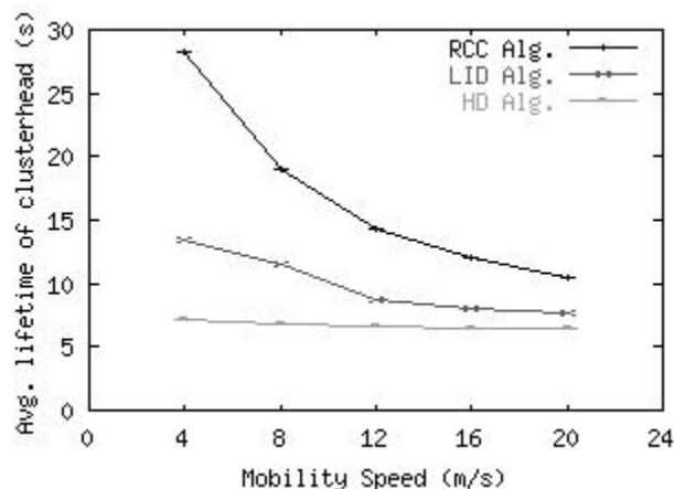
Fig. 3: Average lifetime of cluster heads
