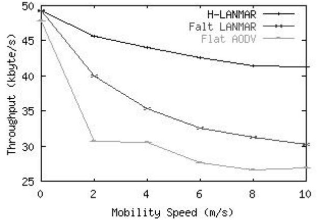
Fig. 8: Comparison of throughput vs. mobility
