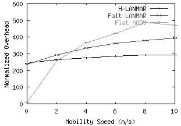
Fig. 10: Comparison of routing overhead vs. mobility
