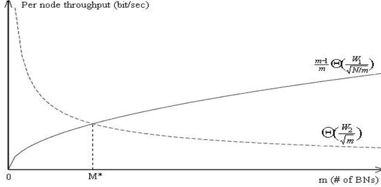
Fig. 2: Throughput as a function of number of BNs
