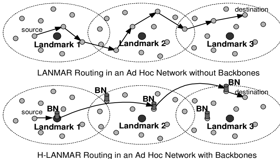
Fig. 6: Illustration of H-LANMAR routing in a MBN
