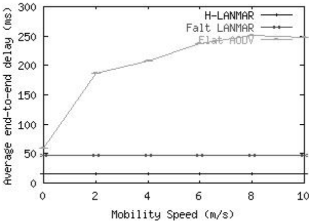
Fig. 9: Comparison of end-to-end delay vs. mobility
