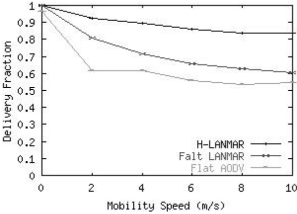
Fig. 7: Comparison of delivery fraction vs. mobility
