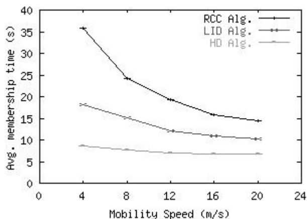
Fig. 4: Average membership time of cluster members
