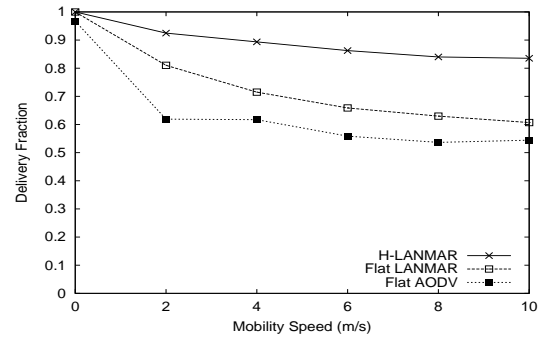
Fig. 5. Comparison of delivery fraction vs. mobility.
