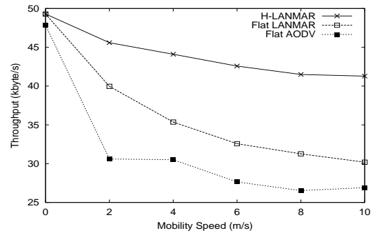
Fig. 6. Comparison of throughput vs. mobility.
