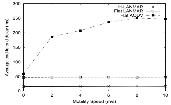
Fig. 7. Comparison of end to end delay vs. mobility.
