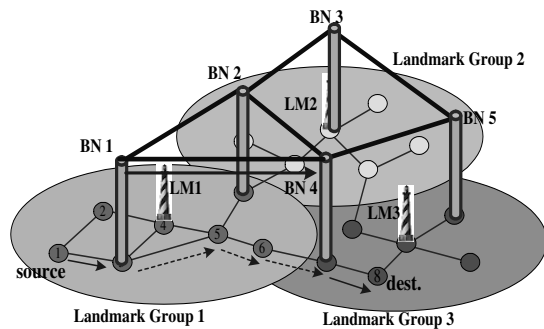
Fig. 4. Illustration of LANMAR routing over mobile backbone network.
