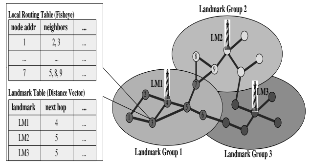
Fig. 3. Illustration of LANMAR routing scheme.
