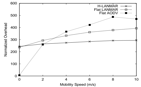
Fig. 8. Comparison of routing overhead vs. mobility.
