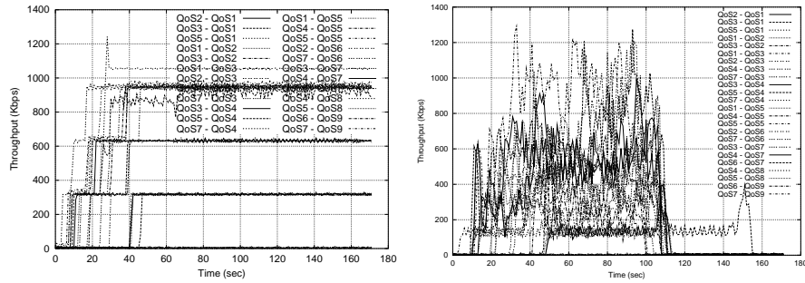
Fig. 9. Throughput profile on every link: CBR: Single Path Fig. 10. Throughput profile on every link: Multimedia: Single Path
