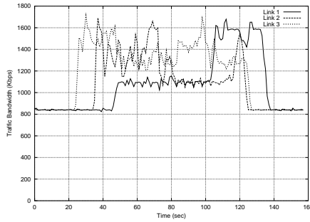
Fig. 7. Throughput profile on the three QPaths: single path
