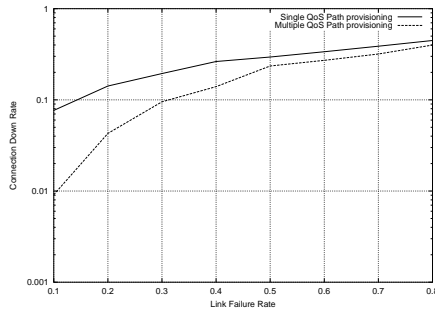
Fig. 12. Connection down rate as a function of link failure rates: CBR
