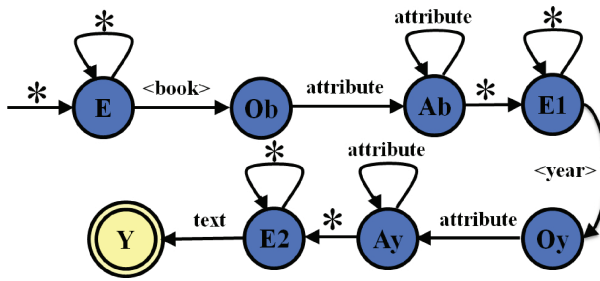
Fig. 7. //book/year/text() .
