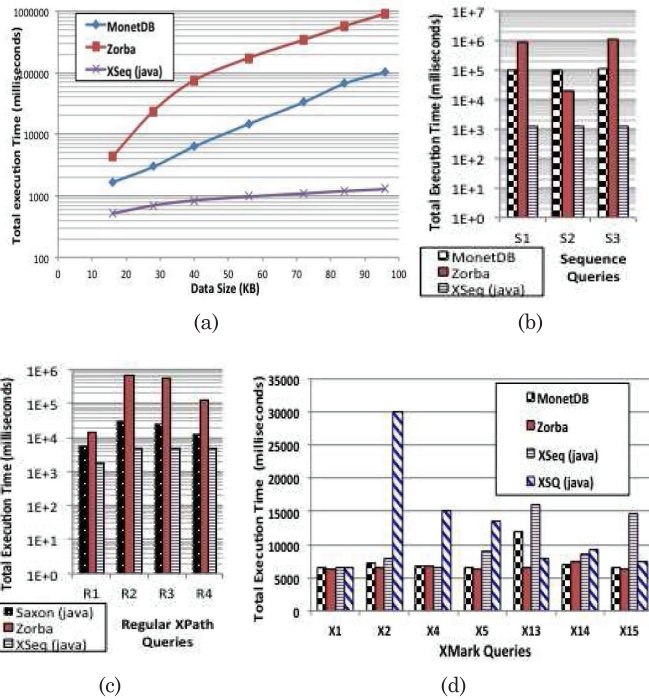
Fig. 10. XSeq vs. XPath/XQuery engines: (a) \nabla -pattern query over Nasdaq stocks; (b) sequence queries over Nasdaq stocks; (c) regular XPath queries over XMark data; (d) conventional XPath queries from XMark.
