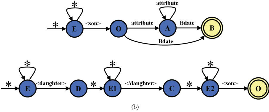
Fig. 5. VPAs for (a) /son@Bdate and (b) /daughter son .
